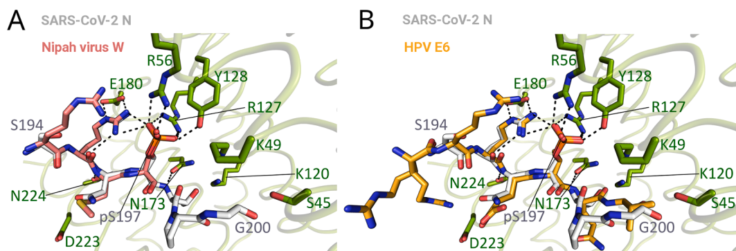
Fig. 2. Superposition of 14-3-3 bound viral peptides. (A) Structural alignment of the SARS-CoV-2N-protein phosphopeptide (white sticks) with phosphopeptide from Nipah virus W protein (PDB ID:6W0L (Edwards et al., 2020)) (Fig. 2A) and bound to the E6 protein of HPV type 18 (PDB ID 6ZFD, (Gogl et al., 2021)) (Fig. 2B) reveals significant differences except for the very conserved central phosphoserine and the arginine residue in the -2 position. (For interpretation of the references to colour in this figure legend, the reader is referred to the web version of this article.)
